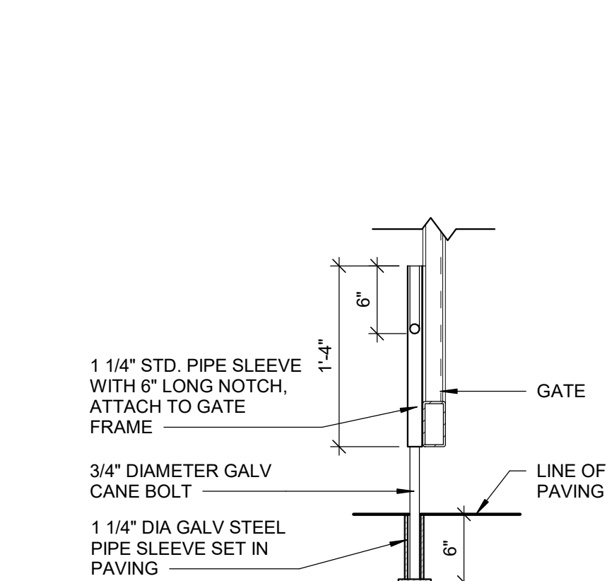
6 SECTION THROUGH GATE
