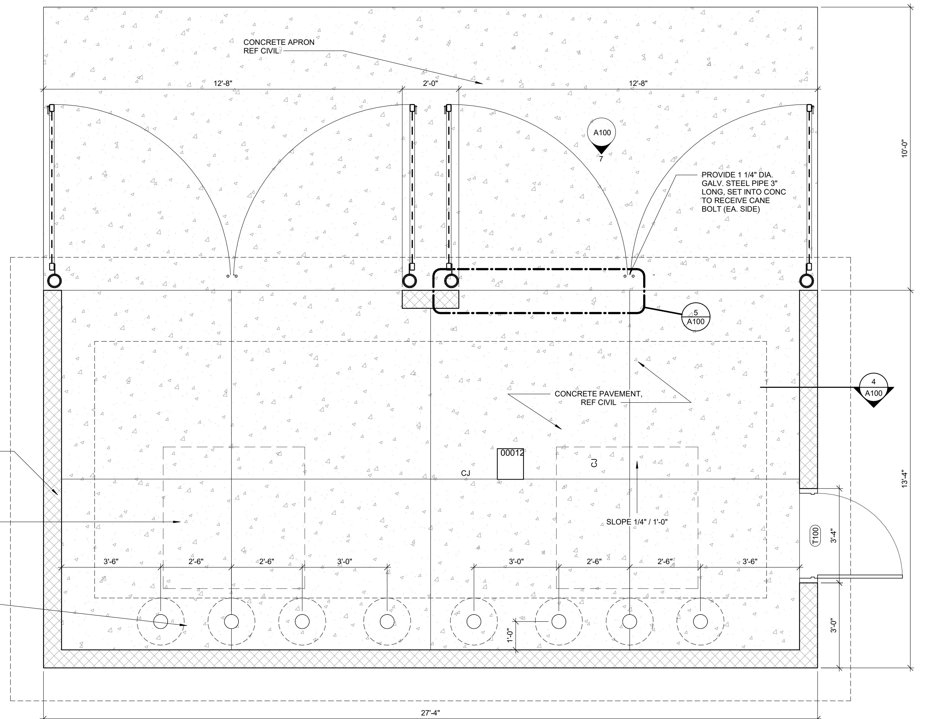
1 TRASH ENCLOSURE PLAN
