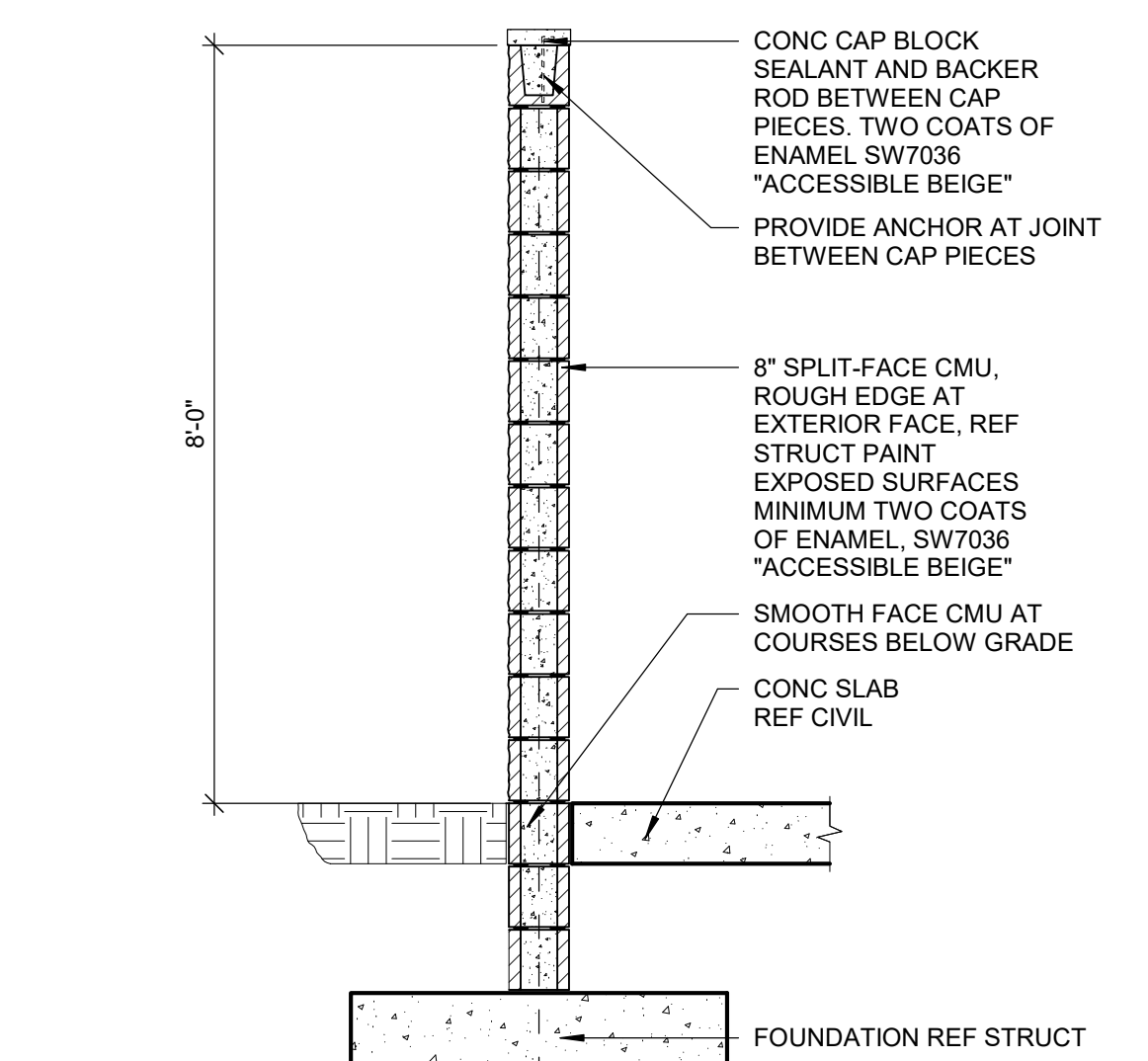
3 TRASH ENCLOSURE WALL SECTION
