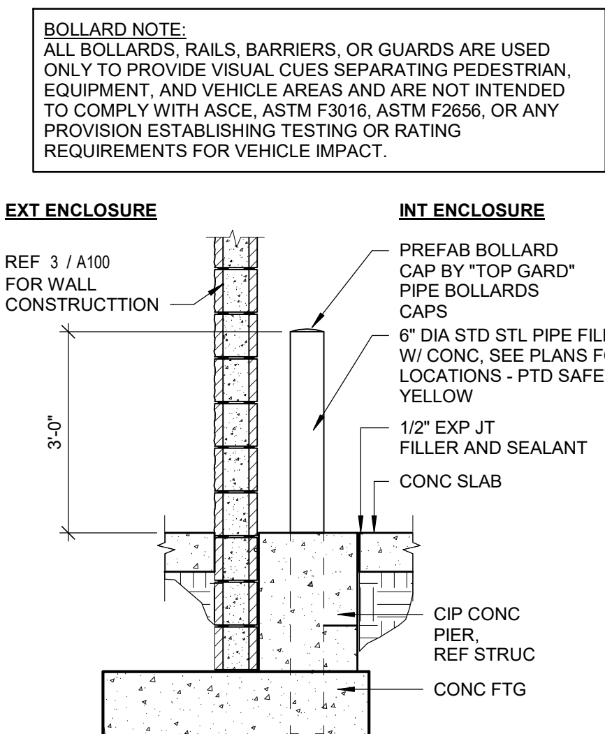
4 PIPE BOLLARD DETAIL
