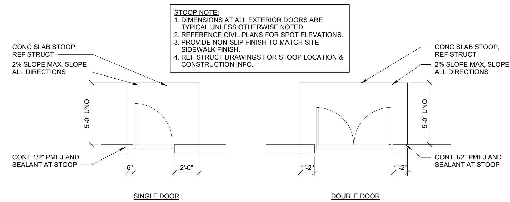
7 STOOP DETAILS
